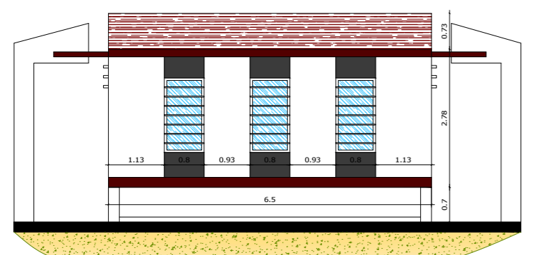
FAÇADE ARRIERE ECH 1 / 50
